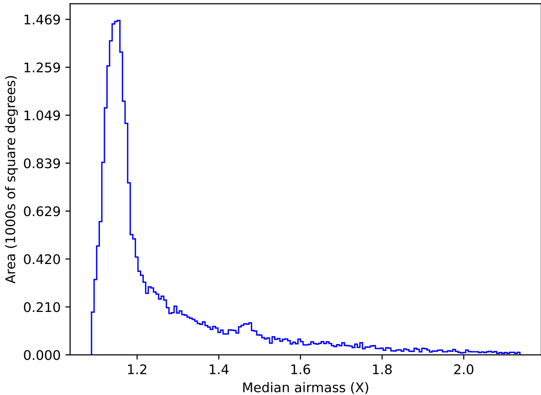
ddf_acor_sf30_lsf40_lsr20_v3.4_10yrs All sky z band: Median airmass
