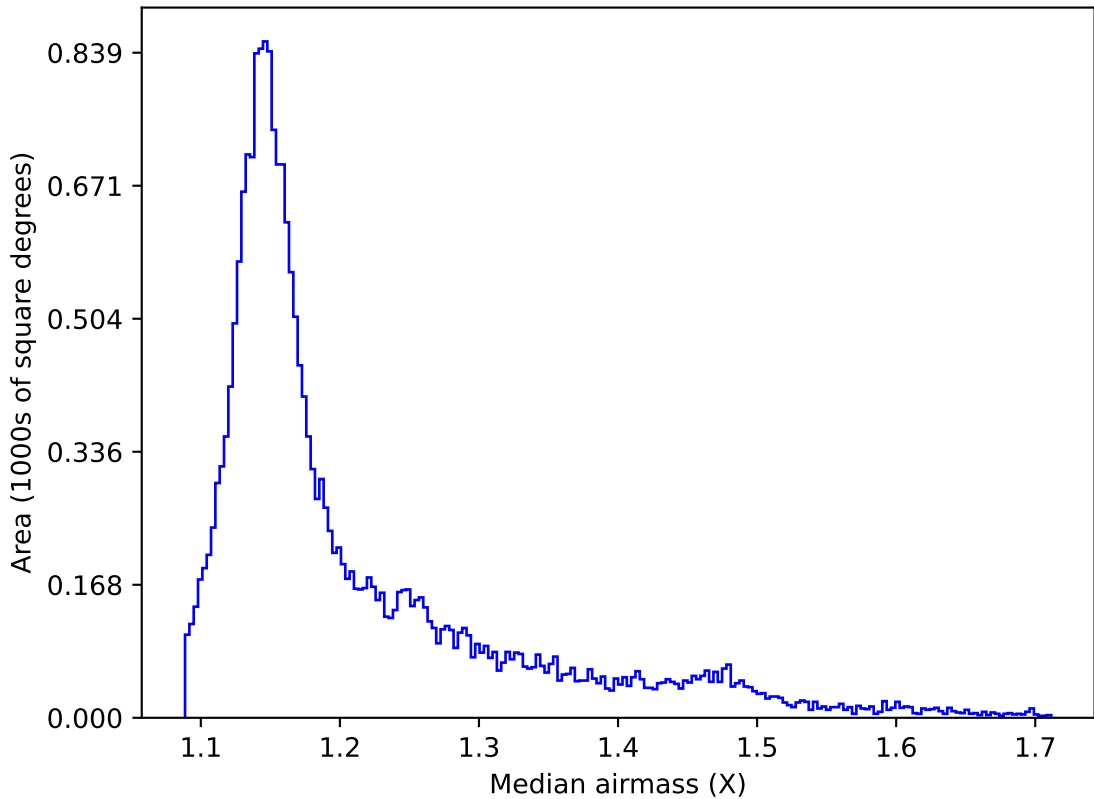
ddf_acor_sf30_lsf40_lsr20_v3.4_10yrs All sky y band: Median airmass
