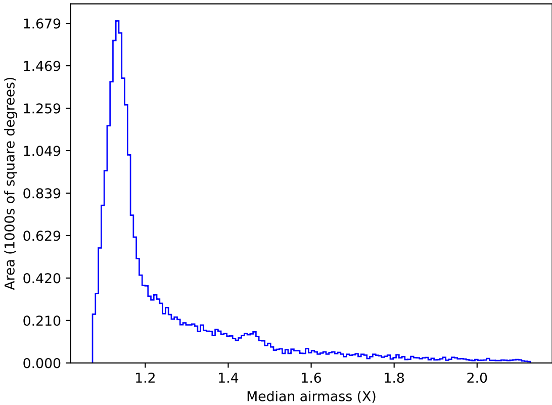
ddf_acor_sf30_lsf40_lsr20_v3.4_10yrs All sky r band: Median airmass
