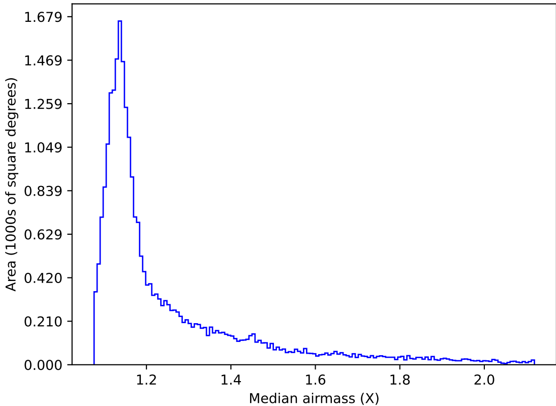
ddf_acor_sf30_lsf40_lsr20_v3.4_10yrs All sky g band: Median airmass
