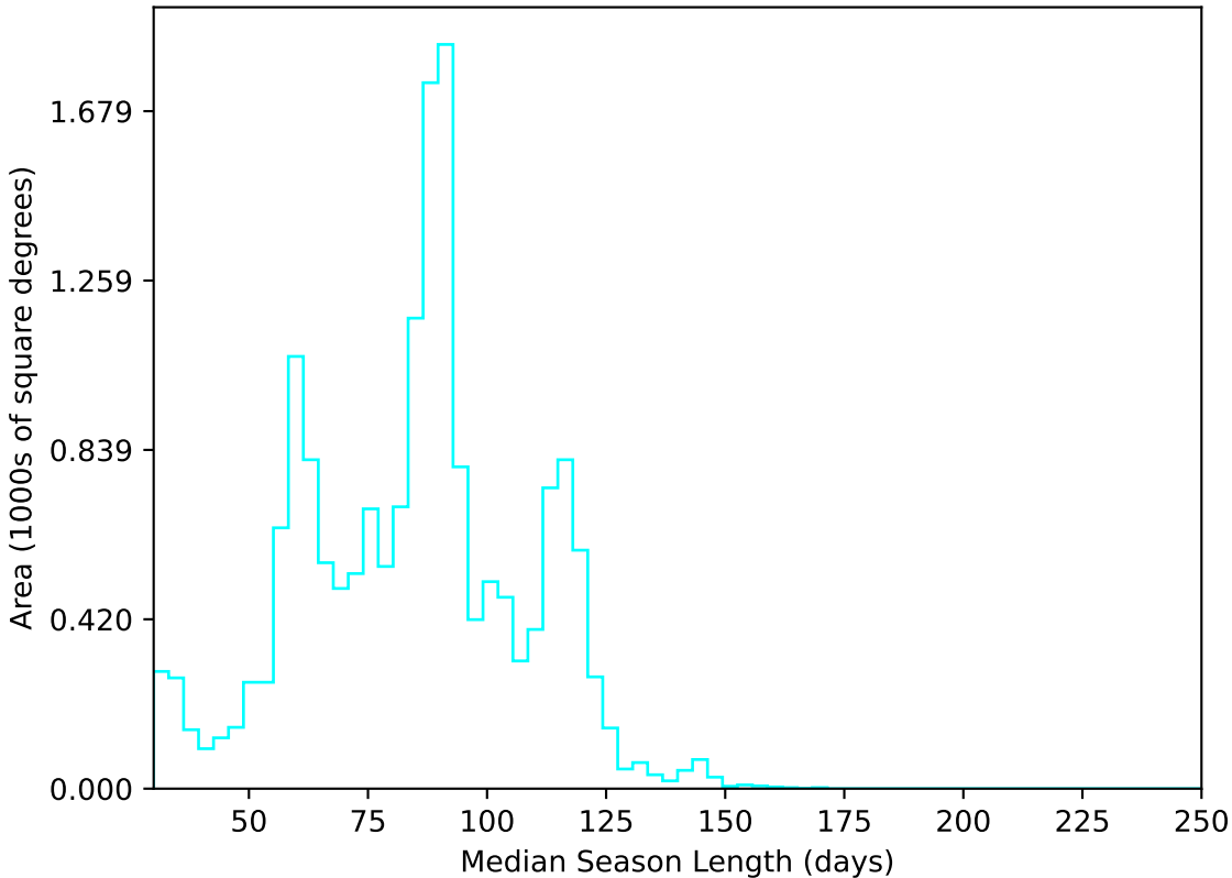
ddf_acor_sf30_lsf40_lsr20_v3.4_10yrs WFD u band: Median Season Length
