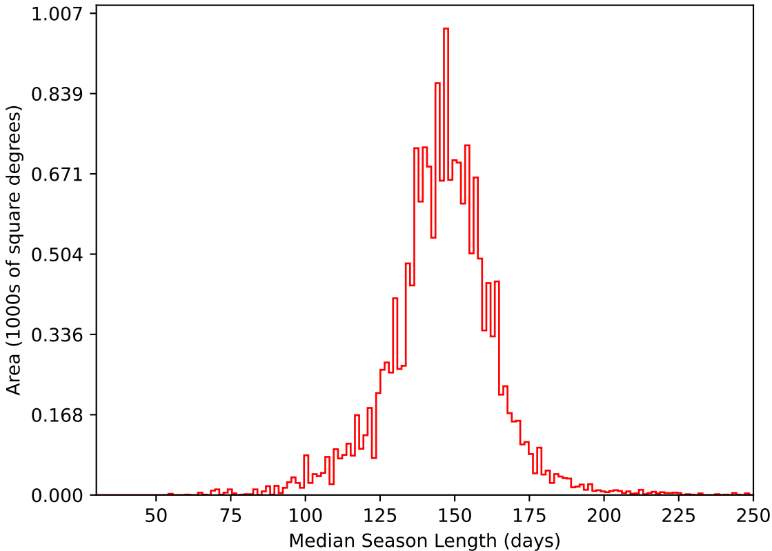
ddf_acor_sf30_lsf40_lsr20_v3.4_10yrs WFD i band: Median Season Length
