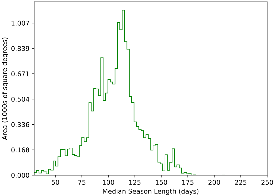
ddf_acor_sf30_lsf40_lsr20_v3.4_10yrs WFD g band: Median Season Length
