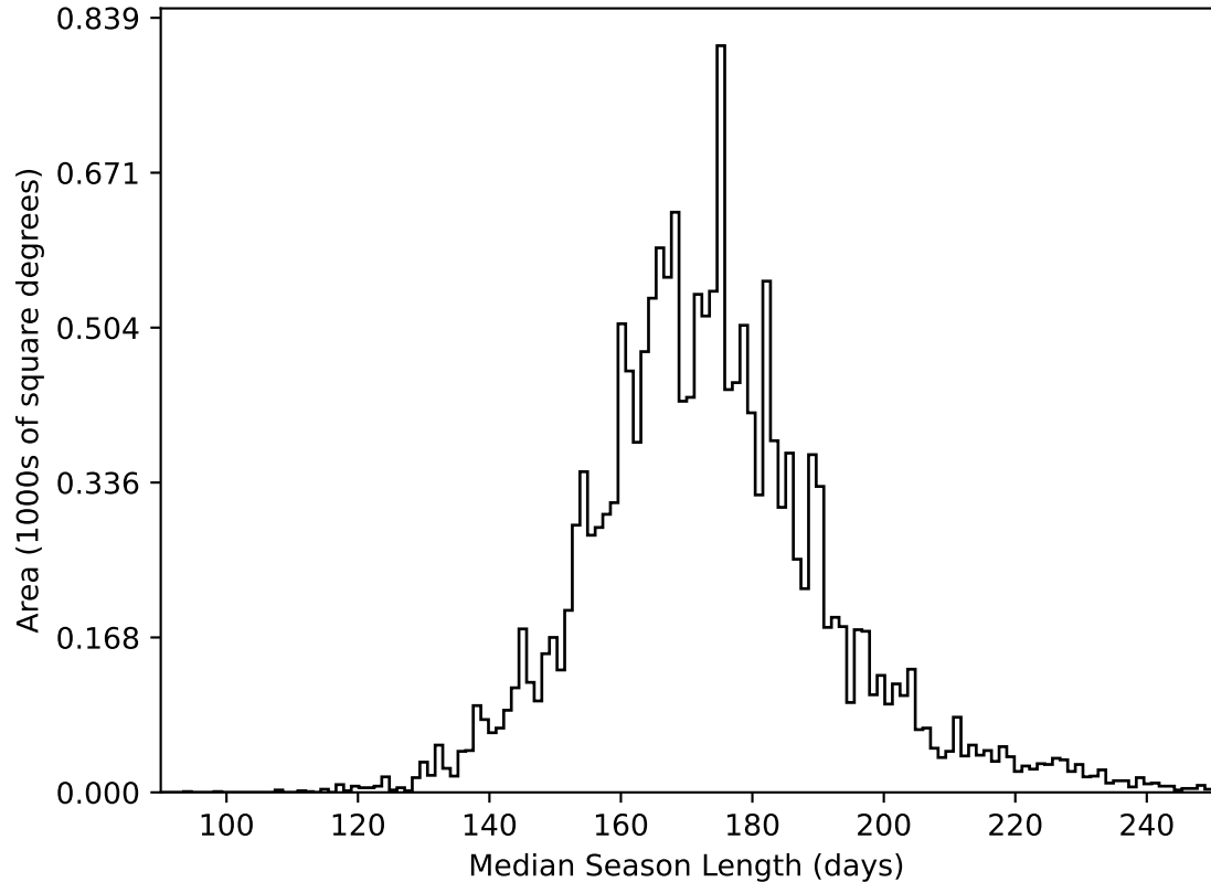
ddf_acor_sf30_lsf40_lsr20_v3.4_10yrs WFD all bands: Median Season Length
