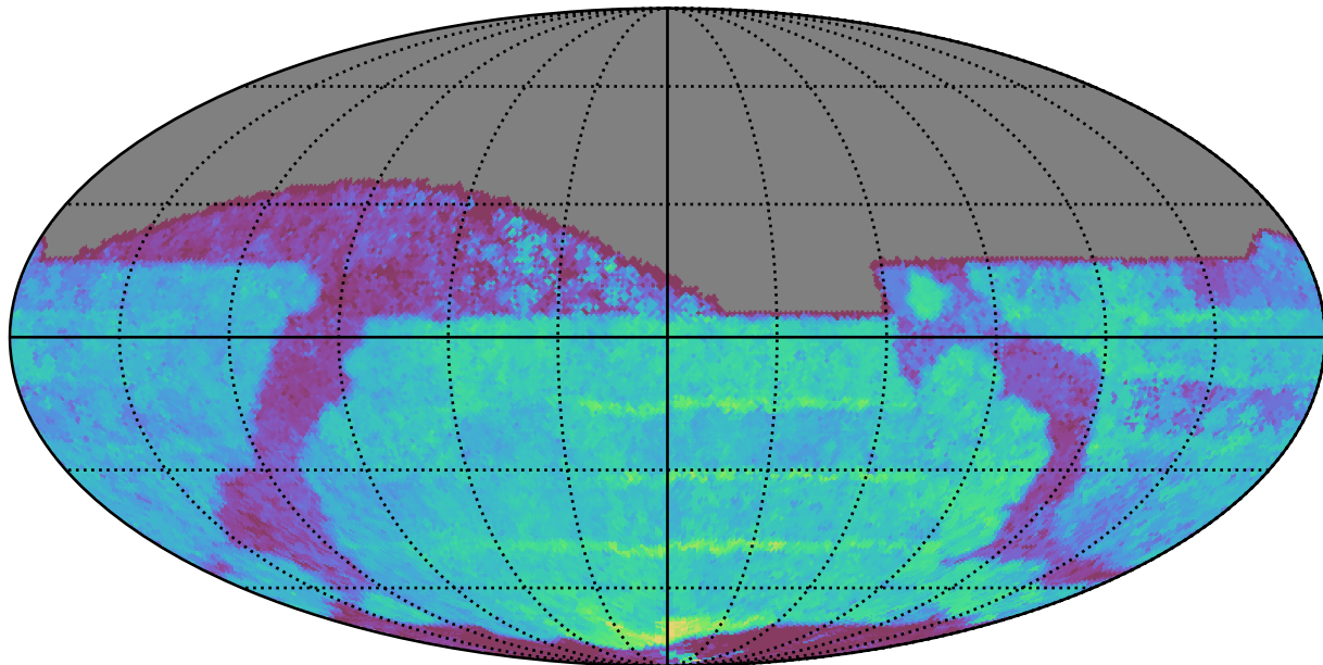
ddf_acor_sf30_lsf40_lsr20_v3.4_10yrs All sky z band: Median Season Length
