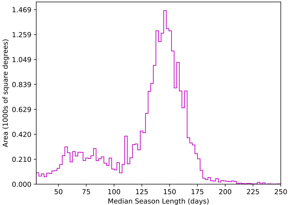
ddf_acor_sf30_lsf40_lsr20_v3.4_10yrs All sky z band: Median Season Length
