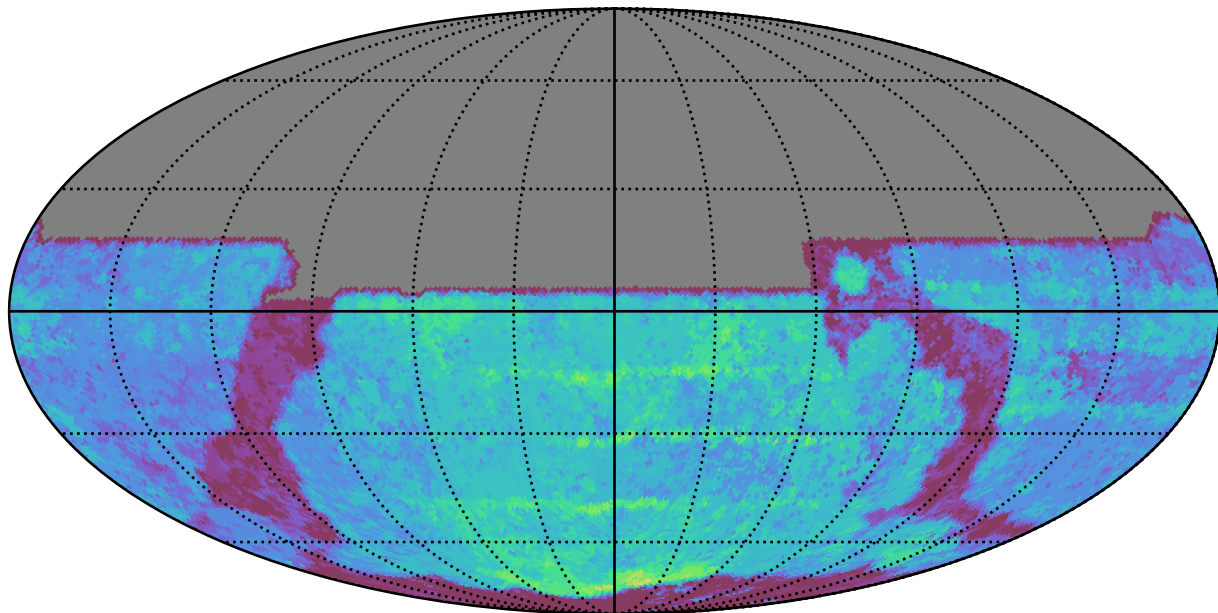
ddf_acor_sf30_lsf40_lsr20_v3.4_10yrs All sky y band: Median Season Length
