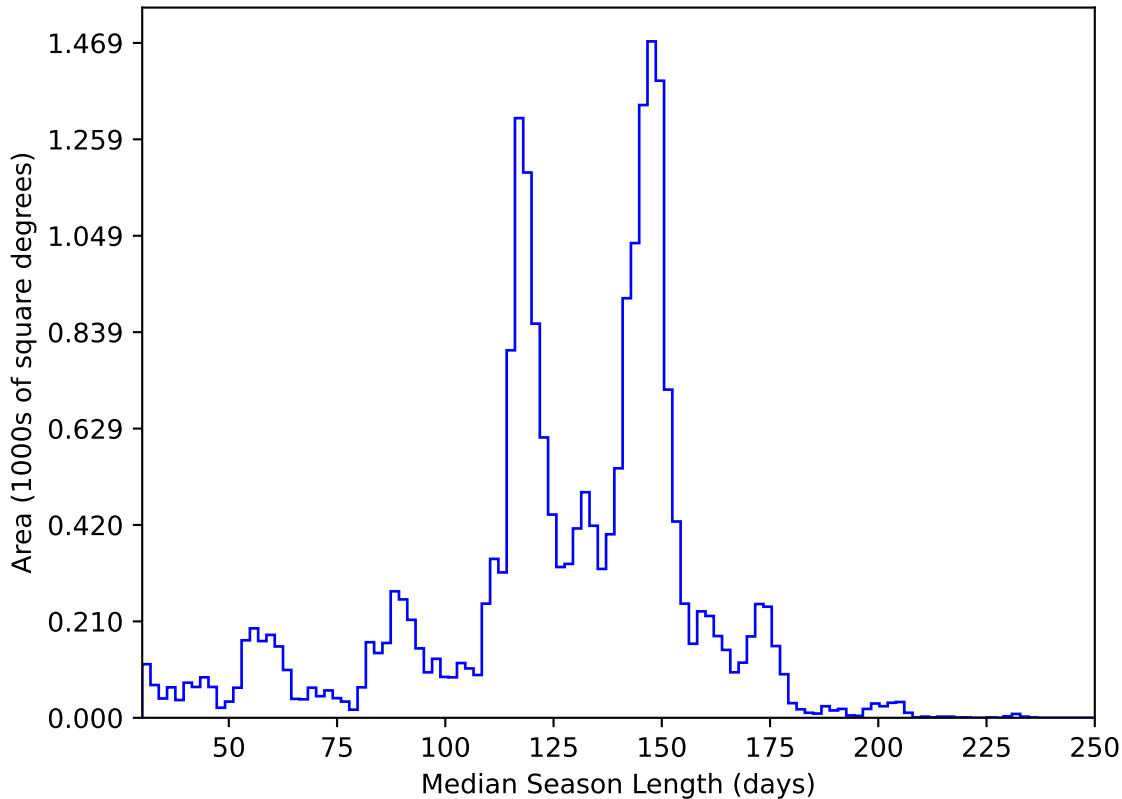
ddf_acor_sf30_lsf40_lsr20_v3.4_10yrs All sky y band: Median Season Length
