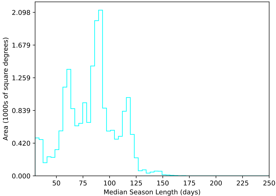
ddf_acor_sf30_lsf40_lsr20_v3.4_10yrs All sky u band: Median Season Length
