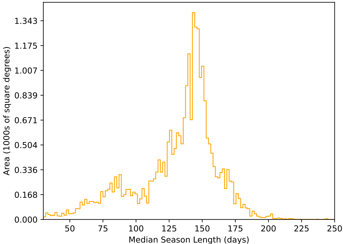
ddf_acor_sf30_lsf40_lsr20_v3.4_10yrs All sky r band: Median Season Length
