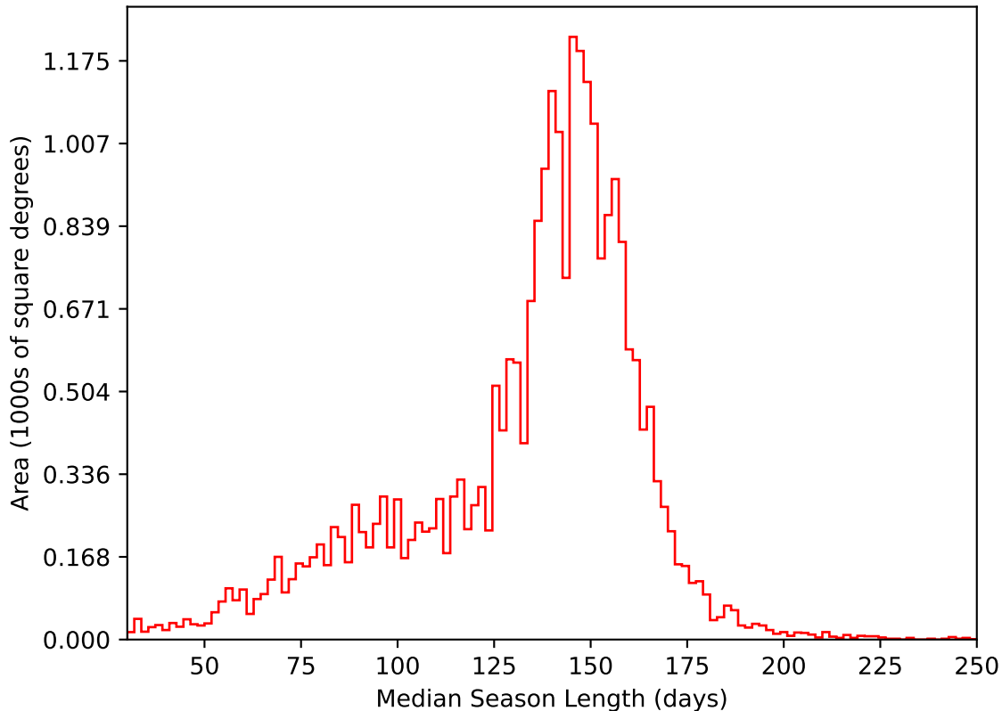
ddf_acor_sf30_Isf40_Isr20_v3.4_10yrs All sky i band: Median Season Length
