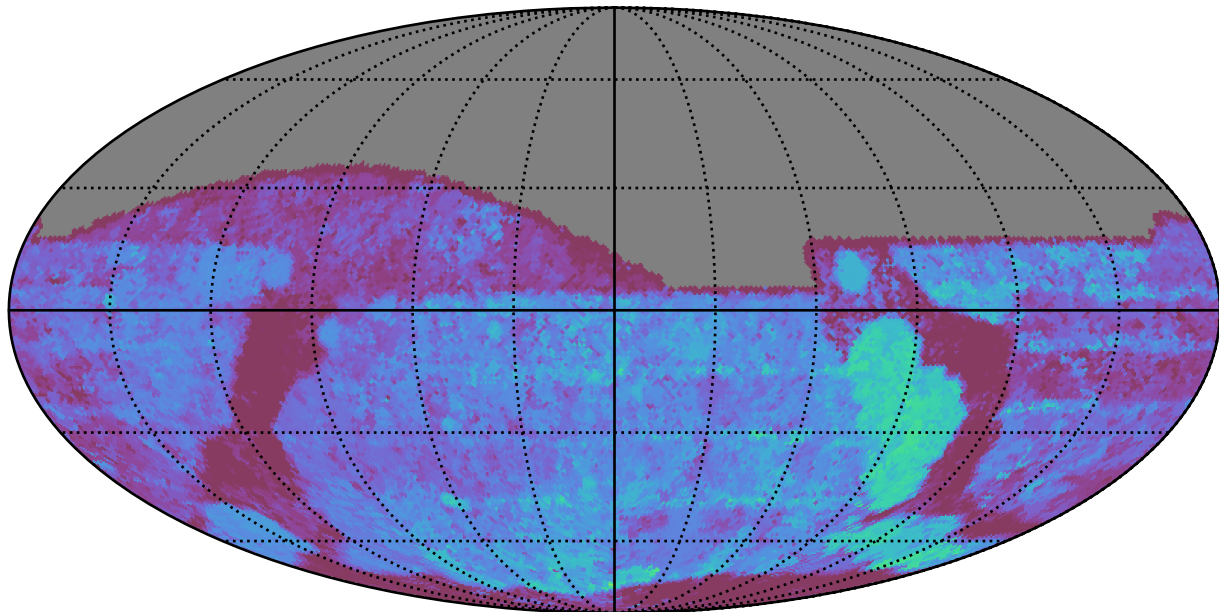
ddf_acor_sf30_lsf40_lsr20_v3.4_10yrs All sky g band: Median Season Length
