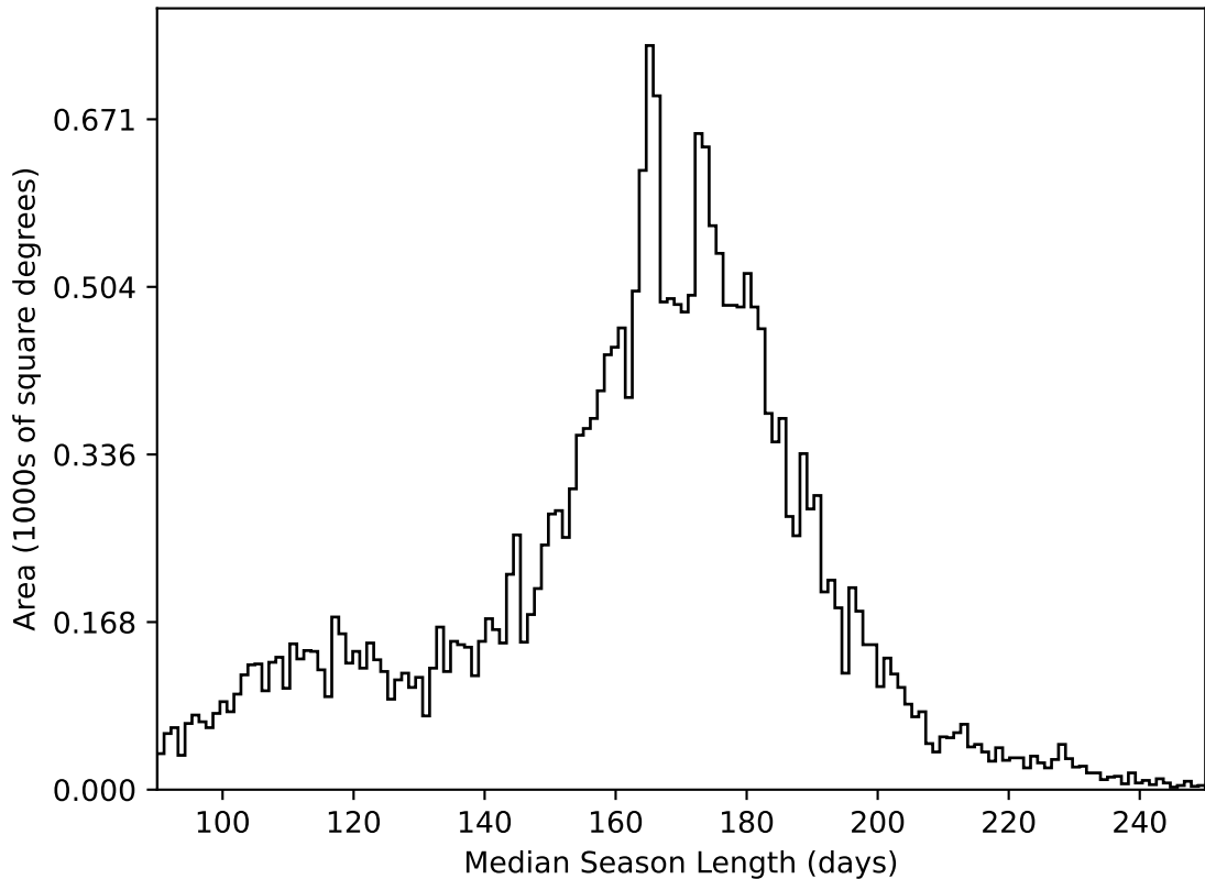
ddf_acor_sf30_lsf40_lsr20_v3.4_10yrs All sky all bands: Median Season Length
