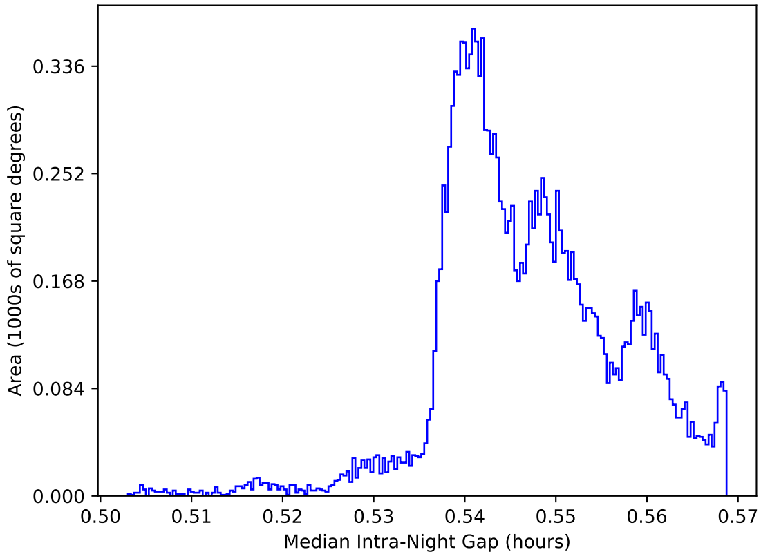
ddf_acor_sf30_ls40_lsr20_v3.4_10yrs WFD: Median Intra-Night Gap
