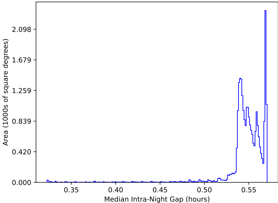
ddf_acor_sf30_lsf40_lsr20_v3.4_10yrs All sky: Median Intra-Night Gap
