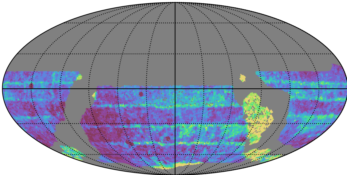
ddf_acor_sf30_lsf40_lsr20_v3.4_10yrs WFD z band: Median Inter-Night Gap
