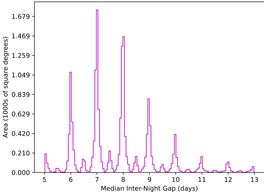
ddf_acor_sf30_lsf40_lsr20_v3.4_10yrs WFD z band: Median Inter-Night Gap
