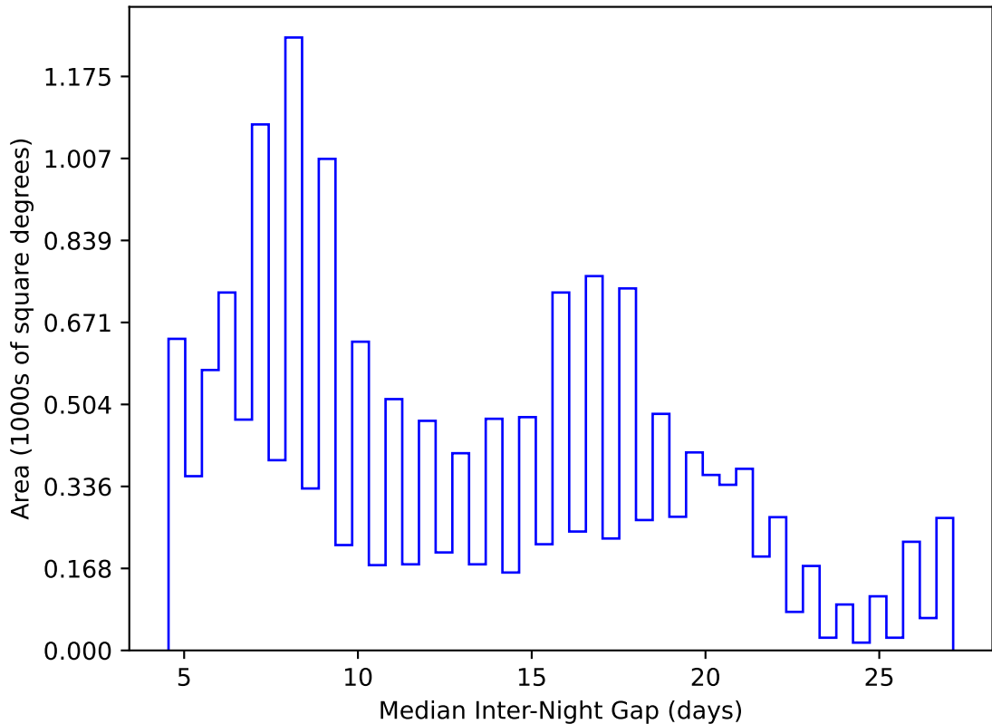
ddf_acor_sf30_lsf40_lsr20_v3.4_10yrs WFD y band: Median Inter-Night Gap
