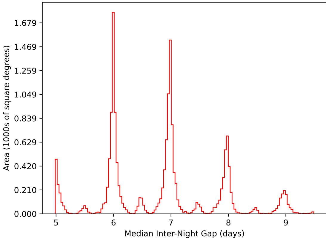
ddf_acor_sf30_lsf40_lsr20_v3.4_10yrs WFD i band: Median Inter-Night Gap
