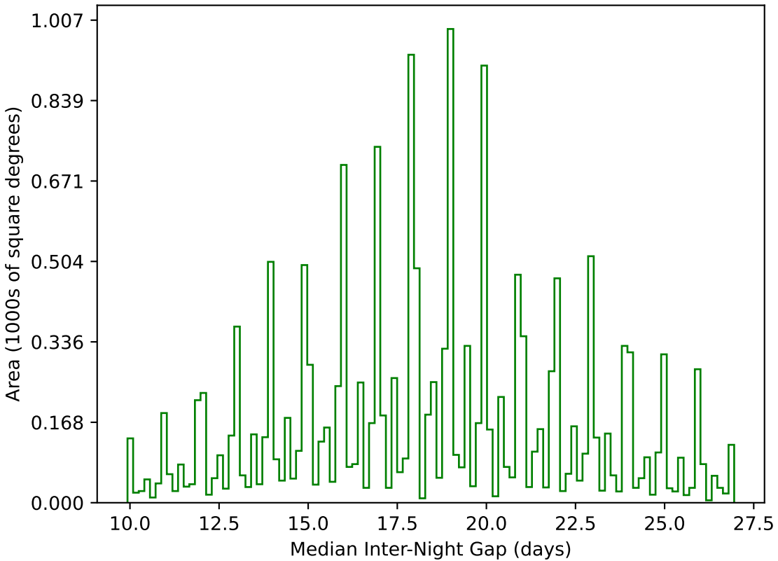
ddf_acor_sf30_lsf40_lsr20_v3.4_10yrs WFD g band: Median Inter-Night Gap
