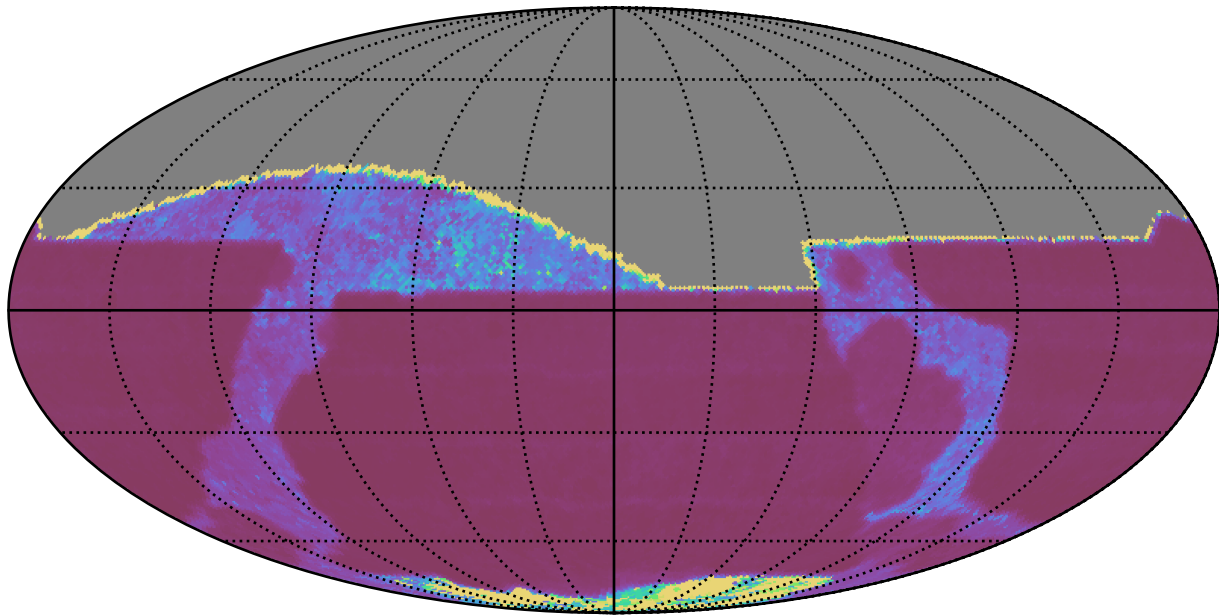
ddf_acor_sf30_lsf40_lsr20_v3.4_10yrs All sky z band: Median Inter-Night Gap
