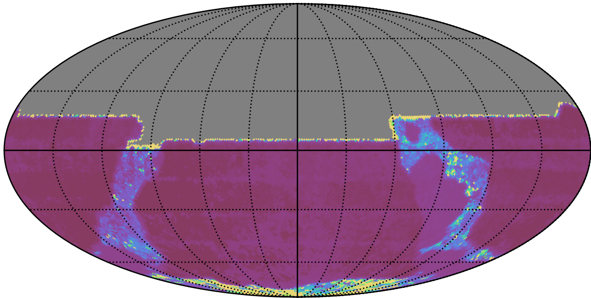
ddf_acor_sf30_lsf40_lsr20_v3.4_10yrs All sky y band: Median Inter-Night Gap
