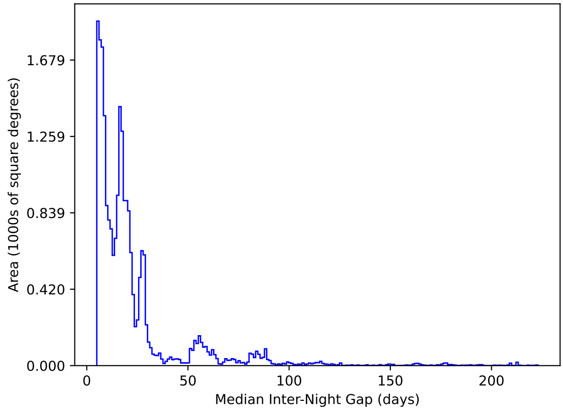
ddf_acor_sf30_lsf40_lsr20_v3.4_10yrs All sky y band: Median Inter-Night Gap
