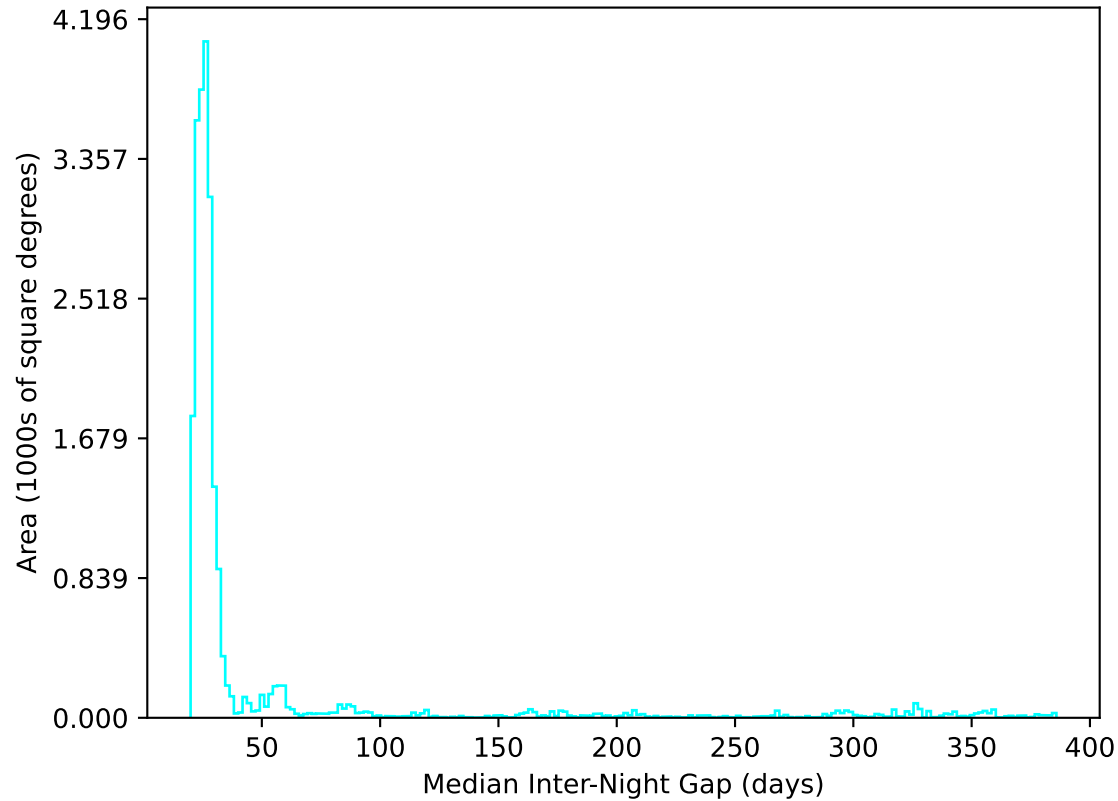
ddf_acor_sf30_lsf40_lsr20_v3.4_10yrs All sky u band: Median Inter-Night Gap
