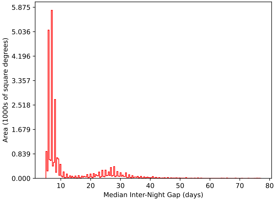
ddf_acor_sf30_lsf40_lsr20_v3.4_10yrs All sky i band: Median Inter-Night Gap
