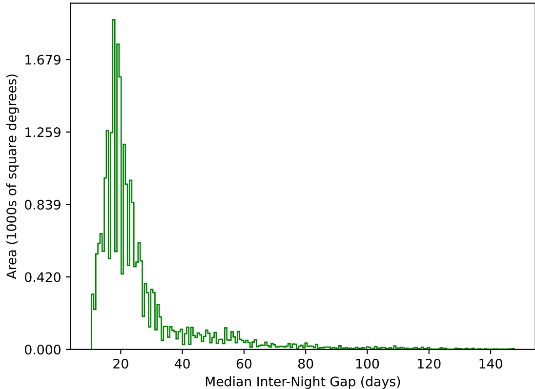
ddf_acor_sf30_lsf40_lsr20_v3.4_10yrs All sky g band: Median Inter-Night Gap
