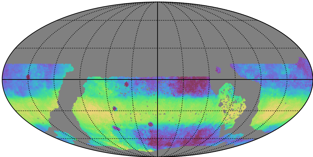
ddf_acor_sf30_lsf40_lsr20_v3.4_10yrs WFD y band: Median HA
