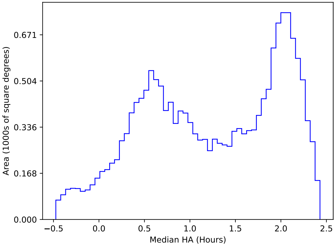
ddf_acor_sf30_lsf40_lsr20_v3.4_10yrs WFD y band: Median HA
