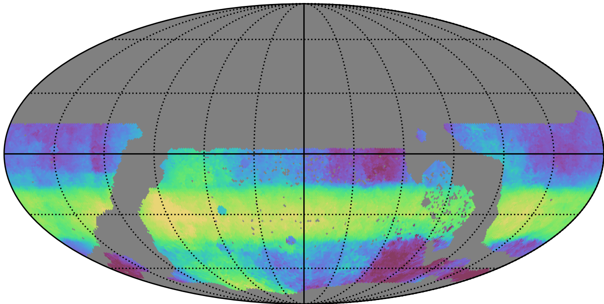
ddf_acor_sf30_lsf40_lsr20_v3.4_10yrs WFD r band: Median HA
