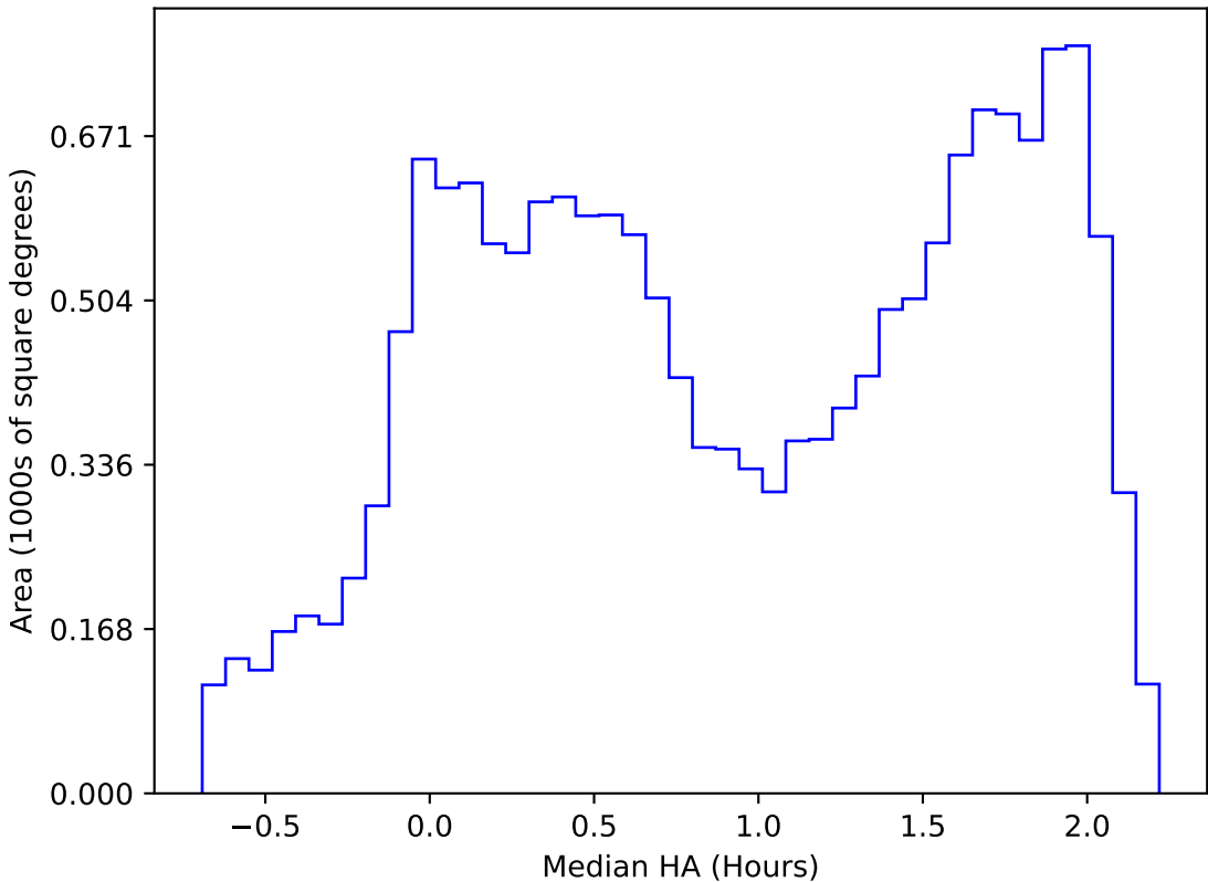
ddf_acor_sf30_lsf40_lsr20_v3.4_10yrs WFD r band: Median HA
