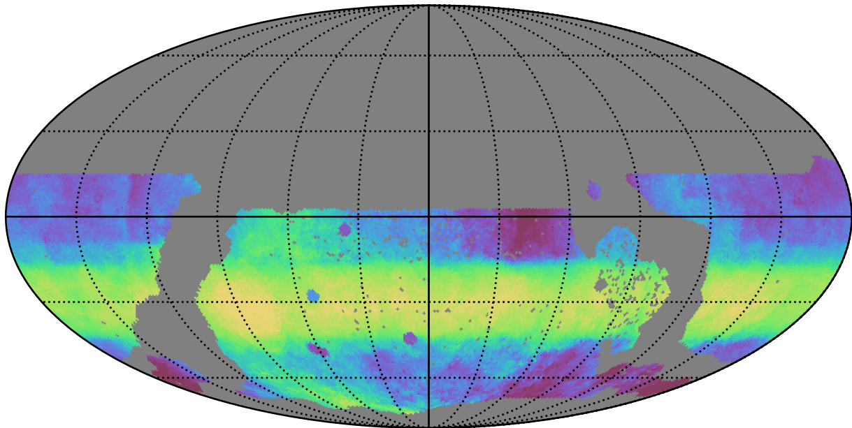
ddf_acor_sf30_lsf40_lsr20_v3.4_10yrs WFD i band: Median HA
