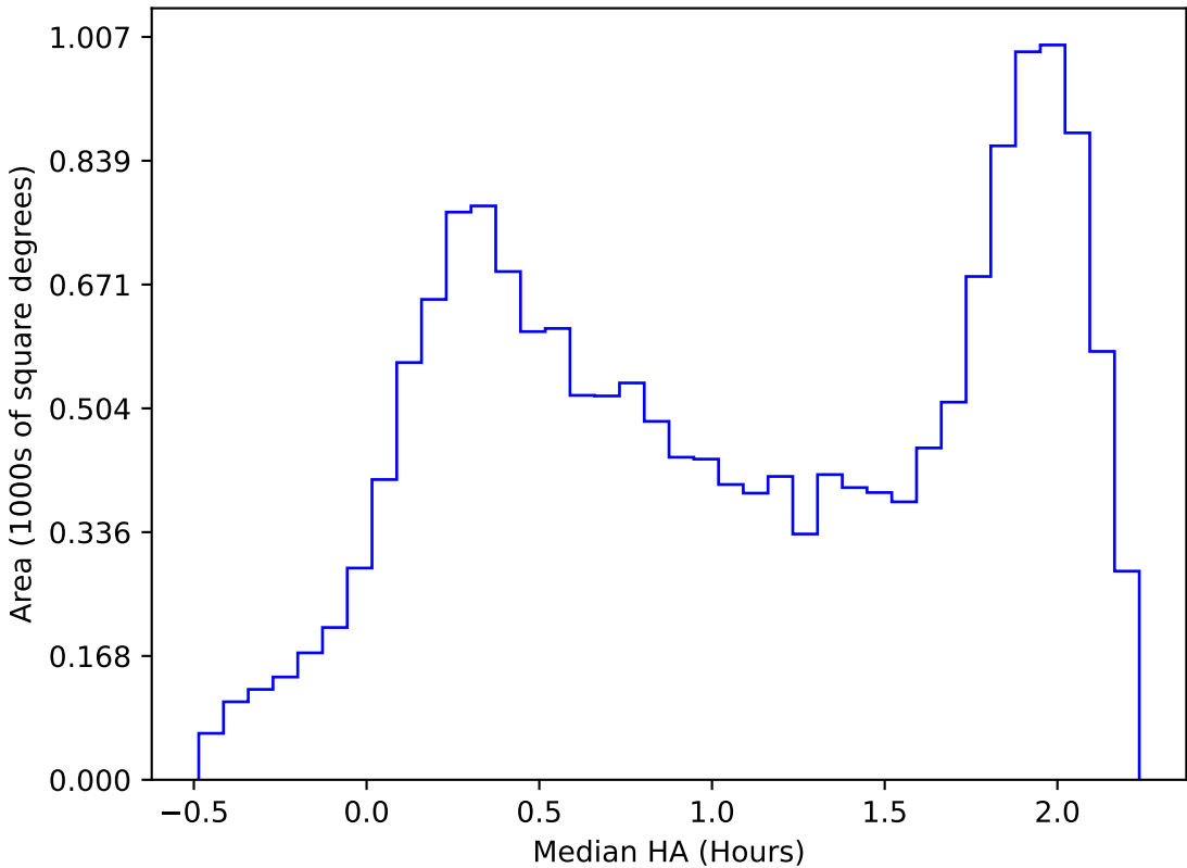
ddf_acor_sf30_lsf40_lsr20_v3.4_10yrs WFD i band: Median HA
