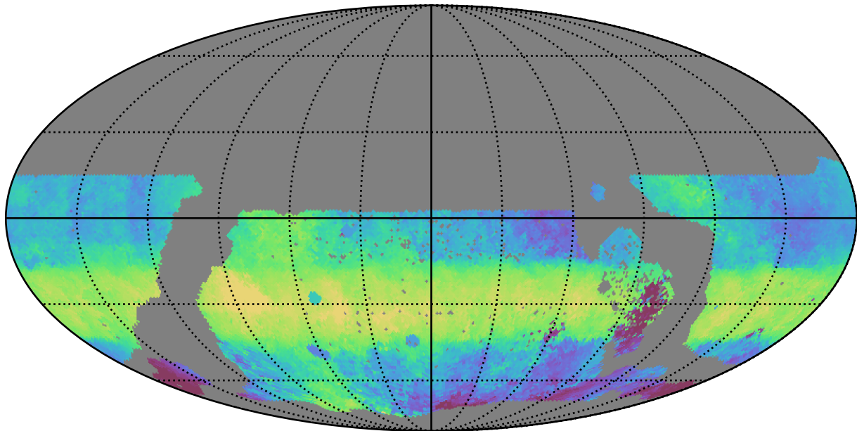
ddf_acor_sf30_lsf40_lsr20_v3.4_10yrs WFD g band: Median HA
