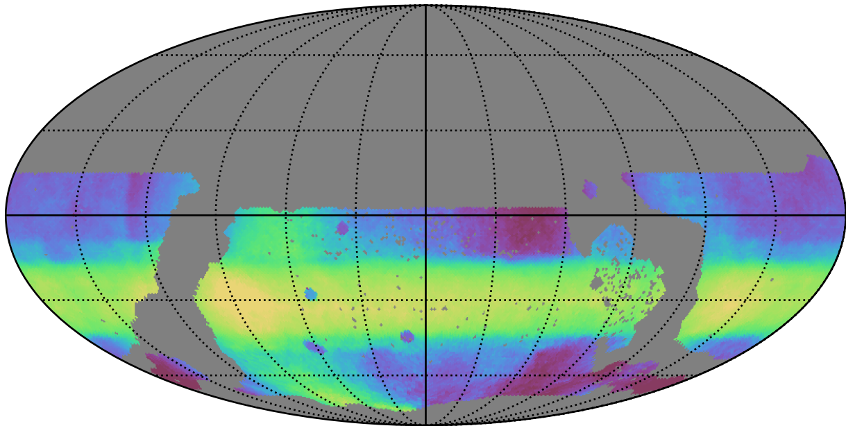
ddf_acor_sf30_lsf40_lsr20_v3.4_10yrs WFD all bands: Median HA
