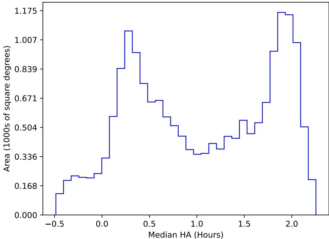
ddf_acor_sf30_lsf40_lsr20_v3.4_10yrs WFD all bands: Median HA
