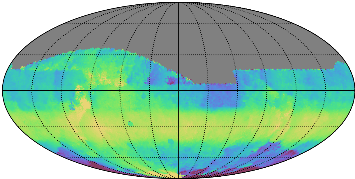
ddf_acor_sf30_lsf40_lsr20_v3.4_10yrs All sky z band: Median HA
