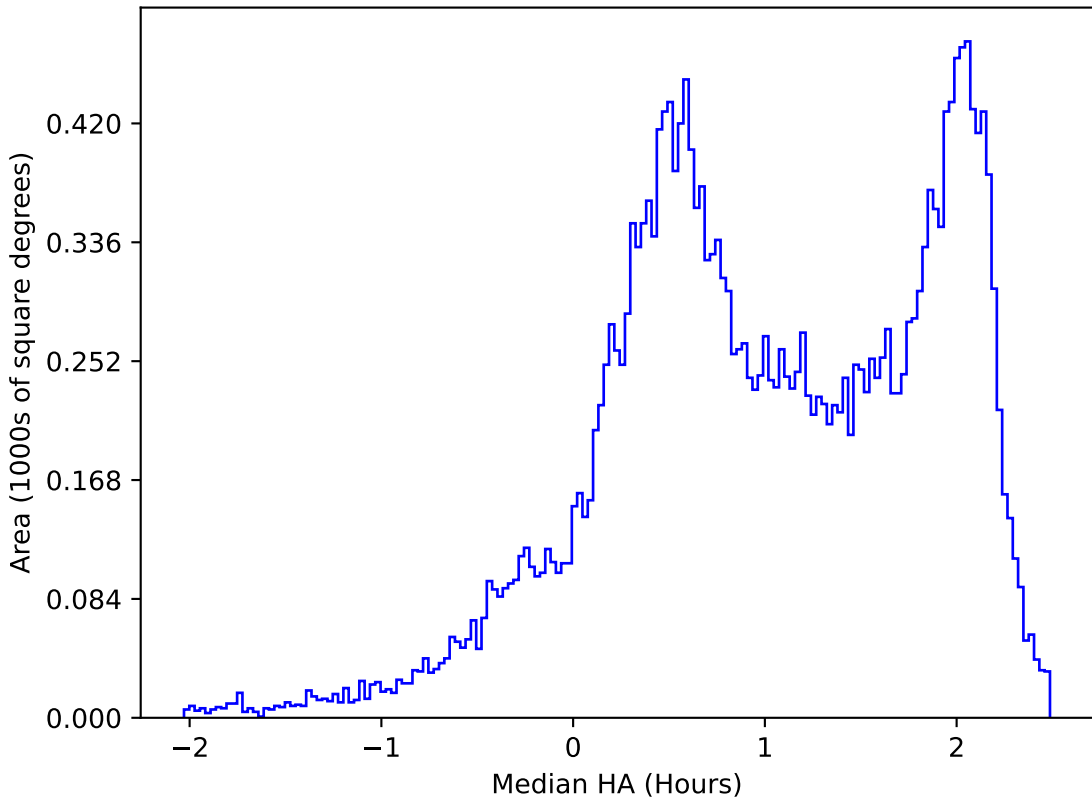
ddf_acor_sf30_lsf40_lsr20_v3.4_10yrs All sky z band: Median HA
