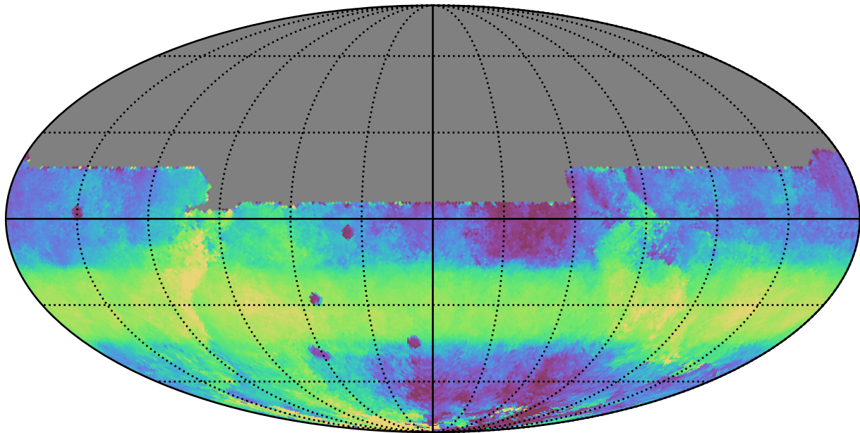
ddf_acor_sf30_lsf40_lsr20_v3.4_10yrs All sky y band: Median HA
