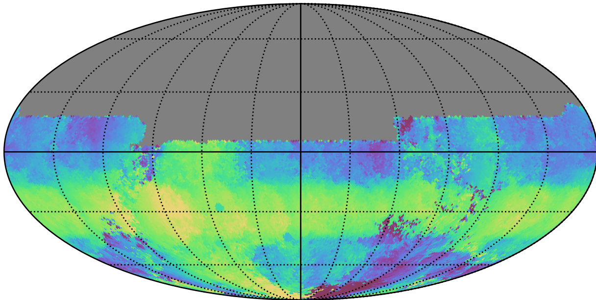
ddf_acor_sf30_lsf40_lsr20_v3.4_10yrs All sky u band: Median HA
