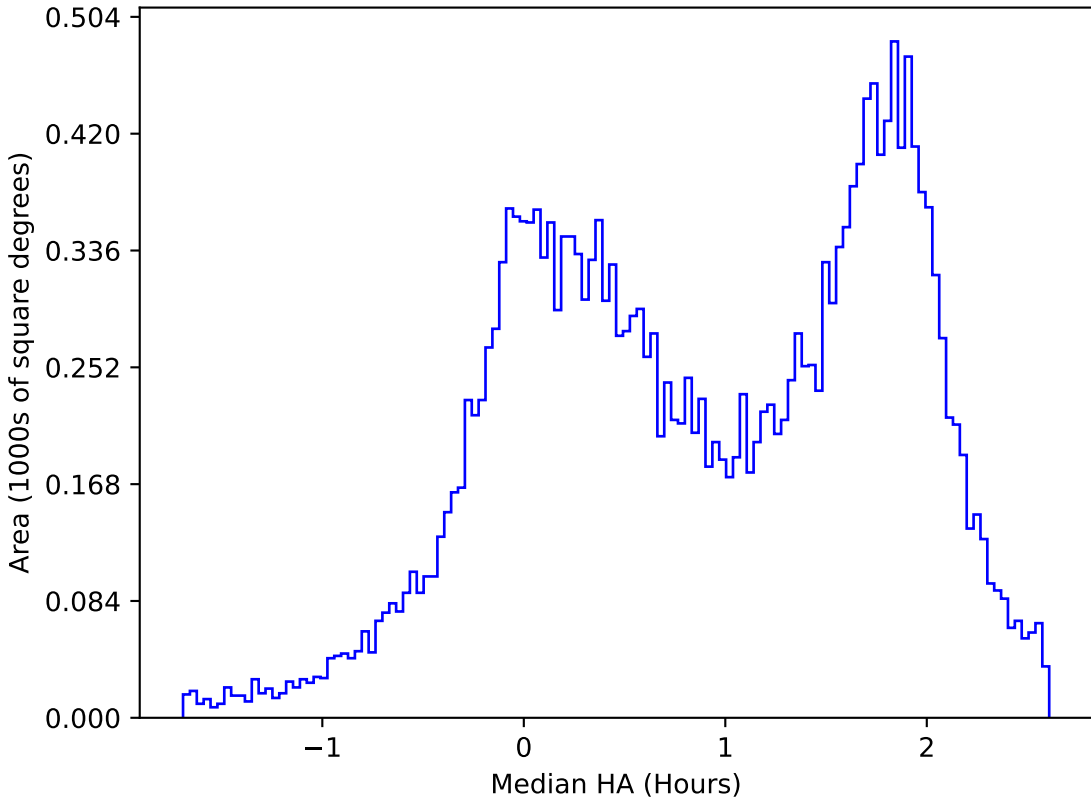
ddf_acor_sf30_lsf40_lsr20_v3.4_10yrs All sky u band: Median HA
