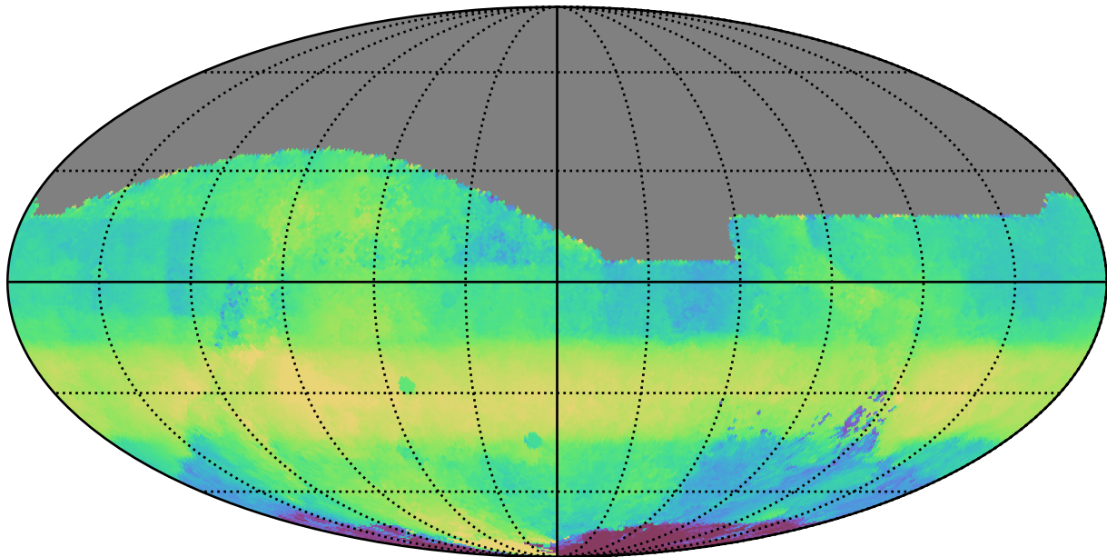
ddf_acor_sf30_lsf40_lsr20_v3.4_10yrs All sky r band: Median HA
