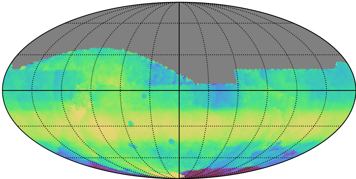
ddf_acor_sf30_lsf40_lsr20_v3.4_10yrs All sky i band: Median HA
