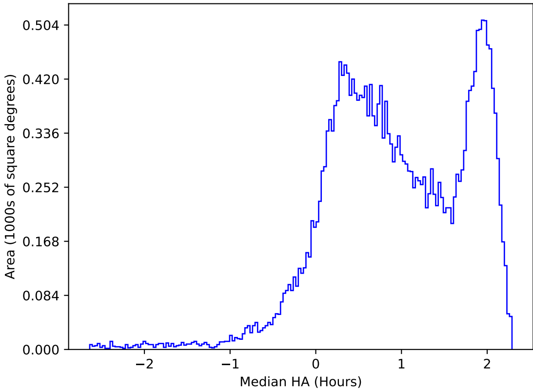
ddf_acor_sf30_lsf40_lsr20_v3.4_10yrs All sky i band: Median HA
