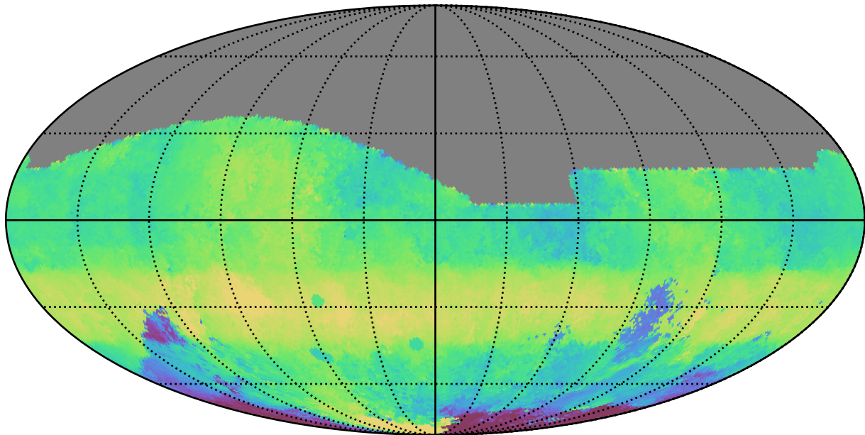
ddf_acor_sf30_lsf40_lsr20_v3.4_10yrs All sky g band: Median HA
