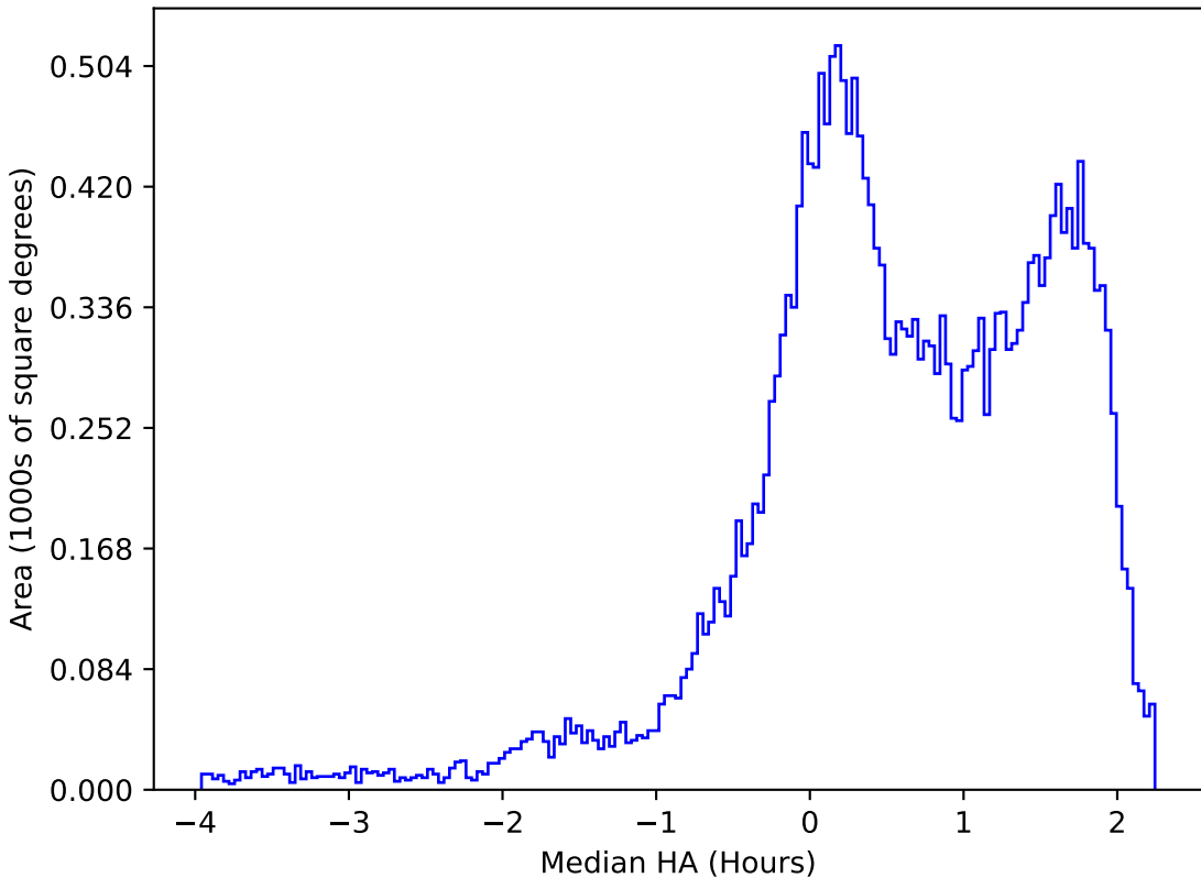
ddf_acor_sf30_lsf40_lsr20_v3.4_10yrs All sky g band: Median HA
