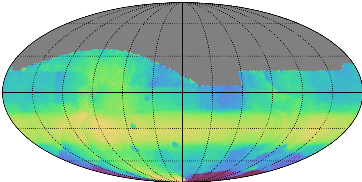
ddf_acor_sf30_lsf40_lsr20_v3.4_10yrs All sky all bands: Median HA
